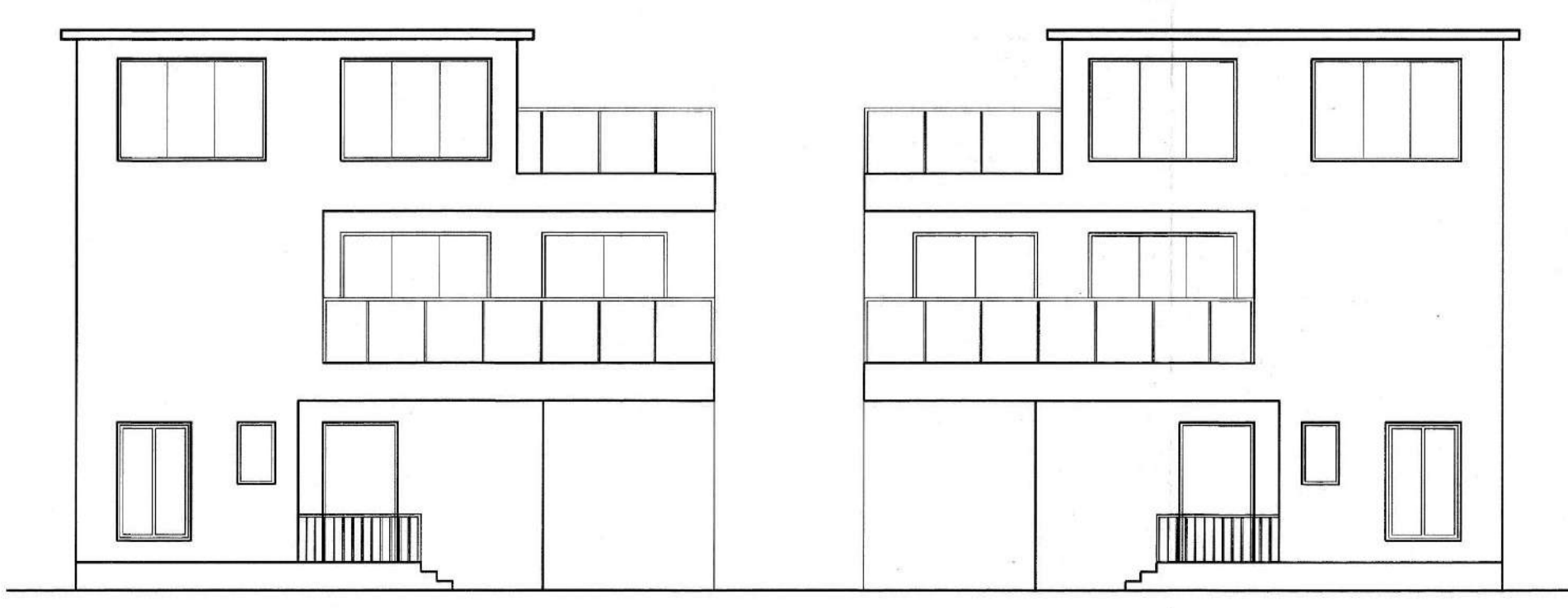
FRONT ELEVATION
