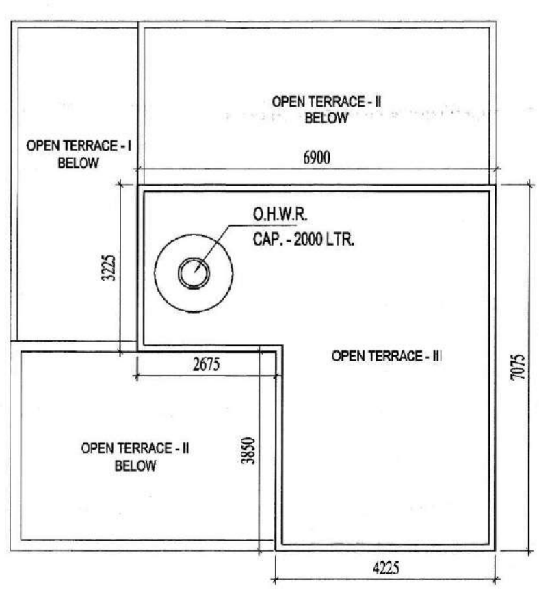
ROOF PLAN
